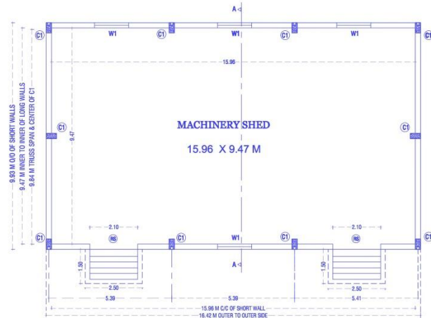
MACHINERY SHED PLAN
